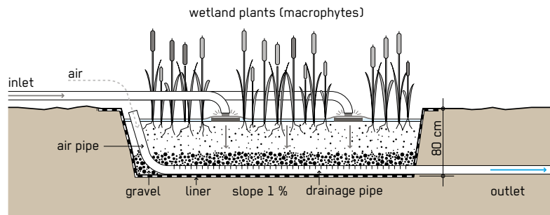
vertical flow constructed wetland
